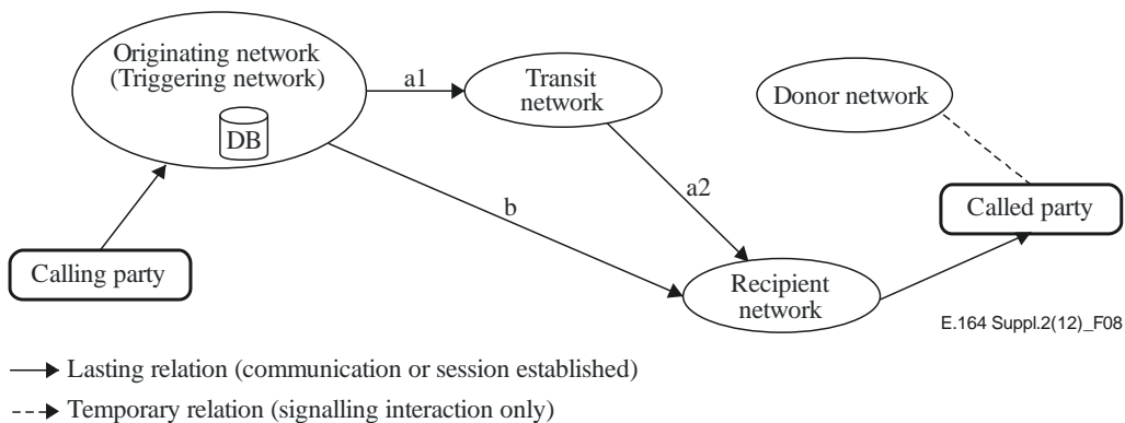
Figure 8 – All call query by originating network
