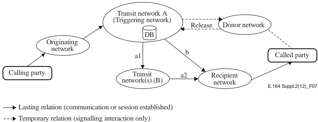
Figure 7 – Query on release by transit network
