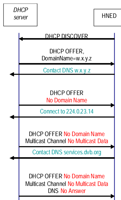
Figure 5.7: SD&S server Entry Point discovery order
